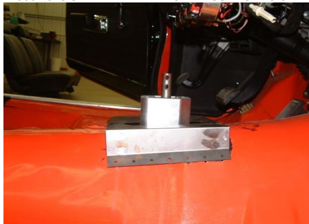
1966-1970 SHEET METAL FROM PASSENGERS SIDE
